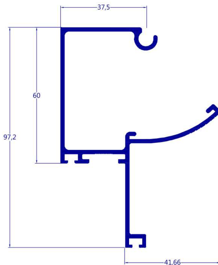
FC-325 1,238 kg/m
